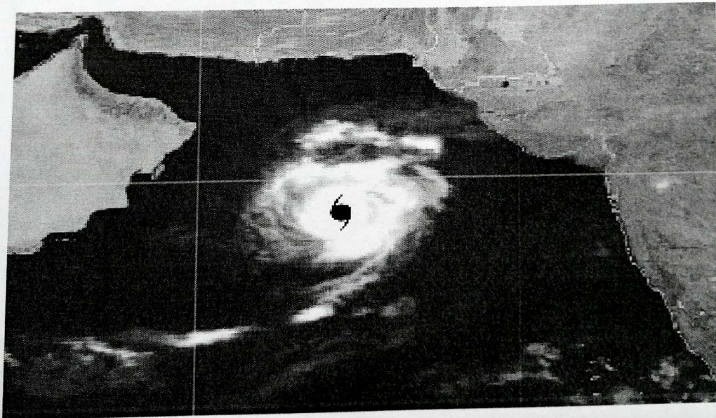
IR Satellite imagery at 1000 PST
