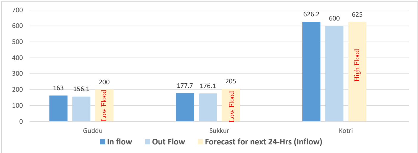
Source: Pakistan Meteorological Department - Flood Forecasting Division (FFD) – Bulletin No. B-089/22 Dated: 11 th September, 2022 10:50 hours (PST)
