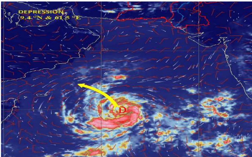
Satellite Imagery, 20 th October 2023, 1430PST
