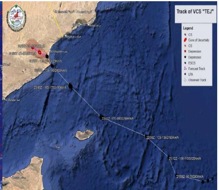
Observed and Forecast Track of Cyclone
