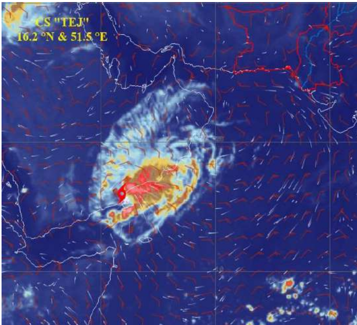
Satellite Imagery, 24 th October 2023, 0930PST
